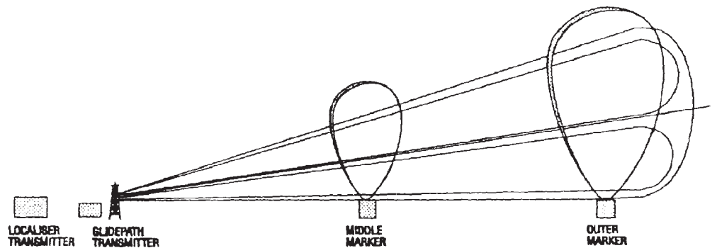
Fig 10-2 Instrument Landing System (ILS)
