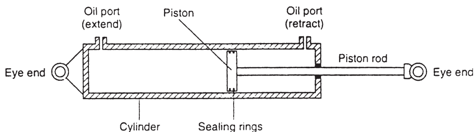
Fig 9-4 Hydraulic Jack
