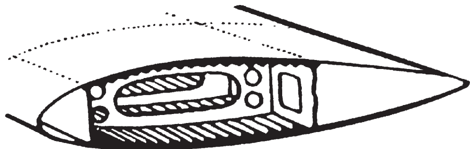
Fig 5-6 Torsion Box Construction
