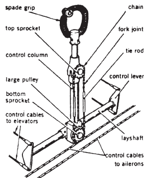
Fig 9-1 Control Column Operation
