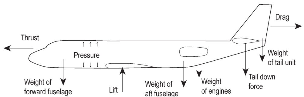
Fig 6-1 Loads on a Fuselage
