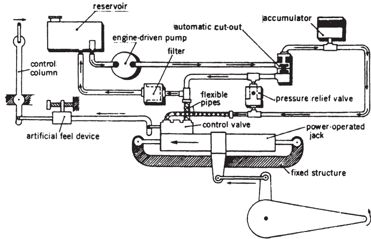
Fig 9-5 Power-Operated Control System
