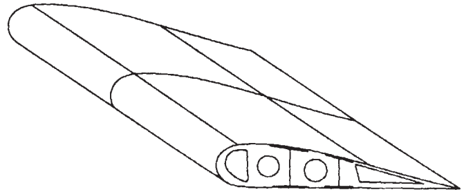
Fig 5-3 More Stressed-Skin Wing Construction
