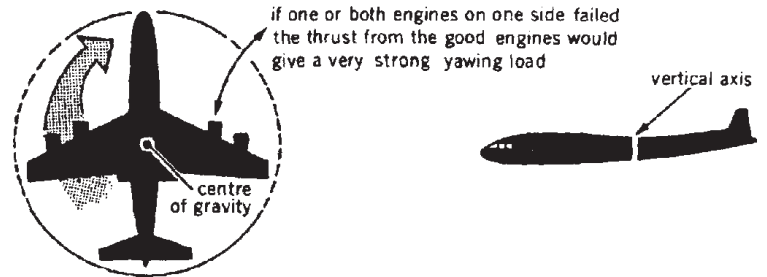
Fig 7-2 Directional Stability
