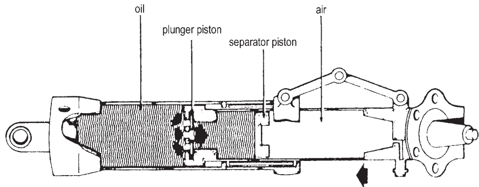
Fig 8-2 Undercarriage Oleo-Pneumatic Leg
