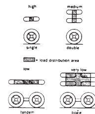
Fig 8-4 Load Distribution Areas
