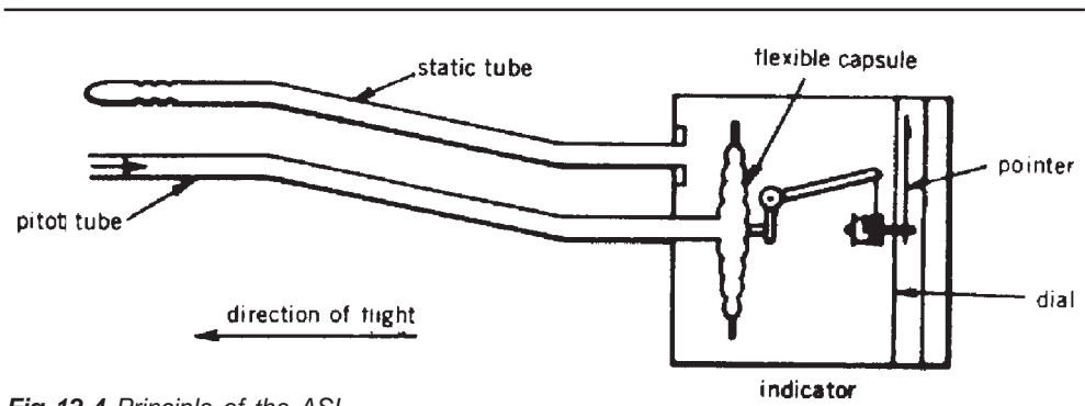
Fig 12-4 Principle of the ASI
