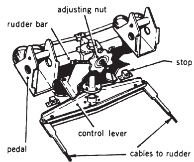
Fig 9-2 Rudder Bar Operation
